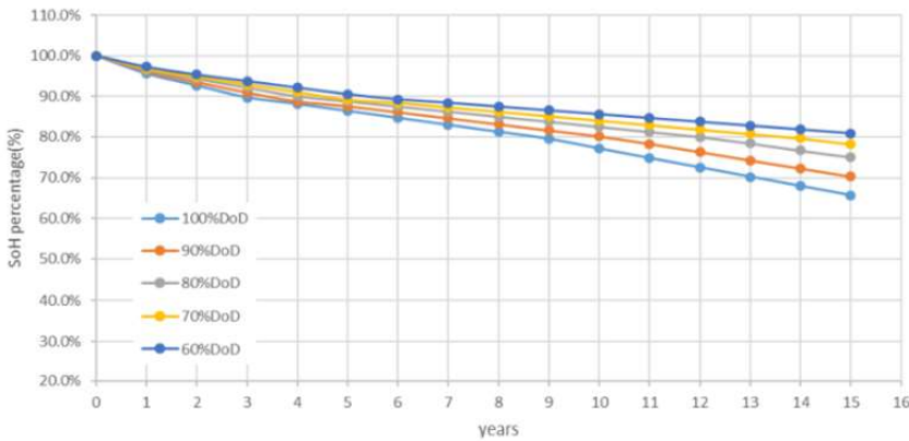
The degradation curve vs different DoD @400cycles/year at 25°C
